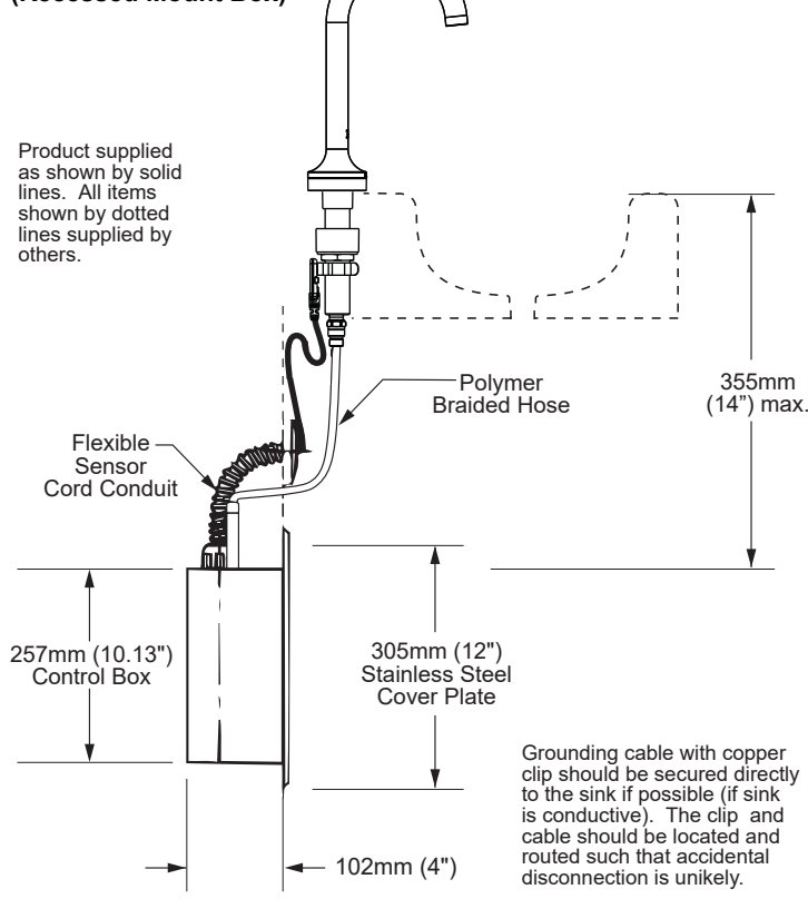
Typical Installation (Recessed Mount Box)
