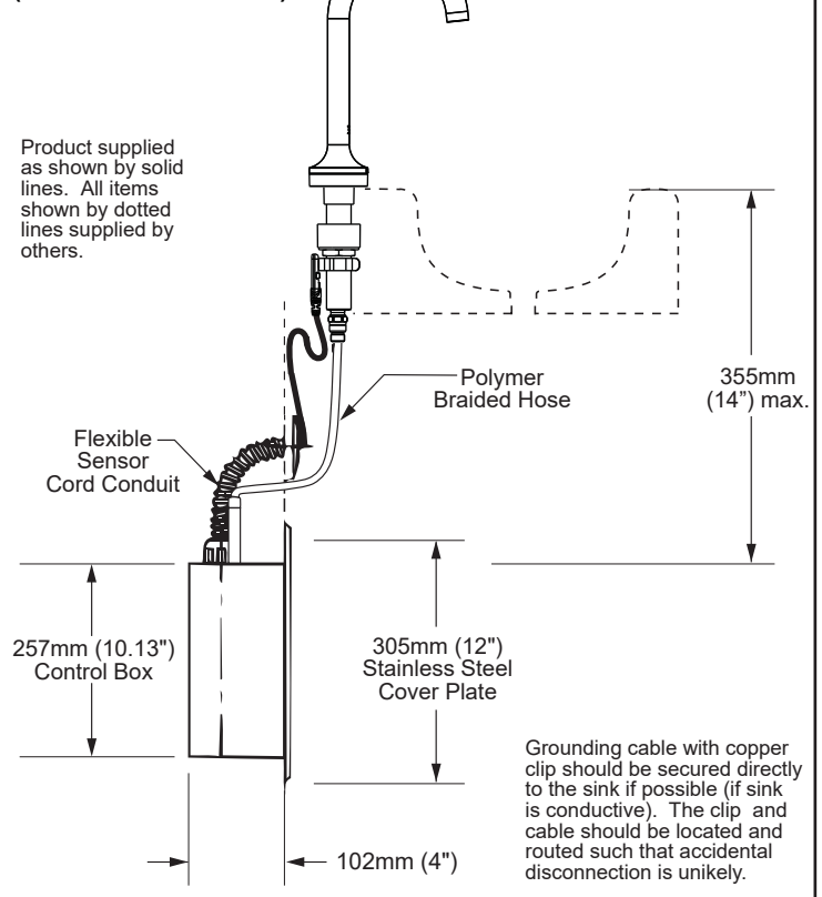
Typical Installation (Recessed Mount Box)
