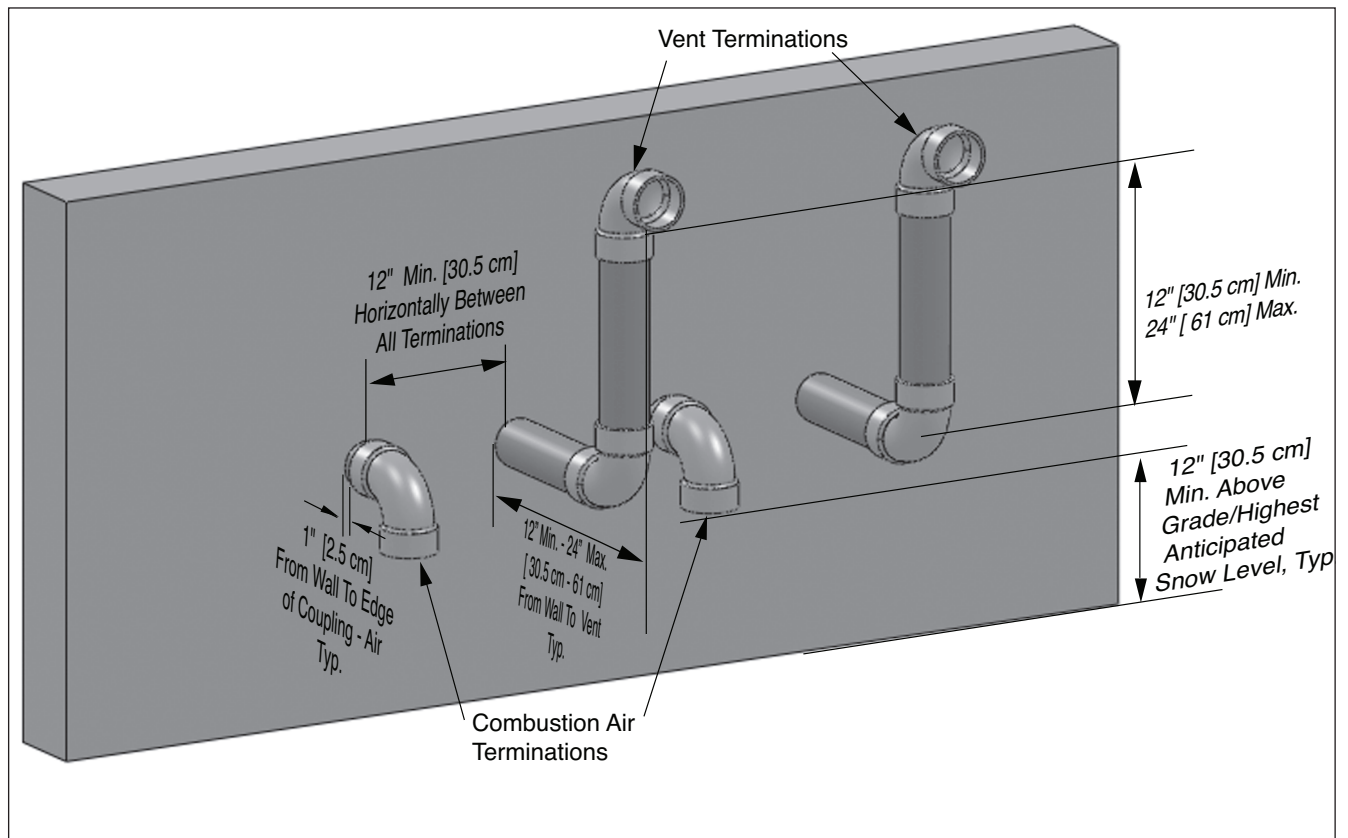
Fig. 11 - Direct Vent - Sidewall Termination of Multiple Prestige Boilers
