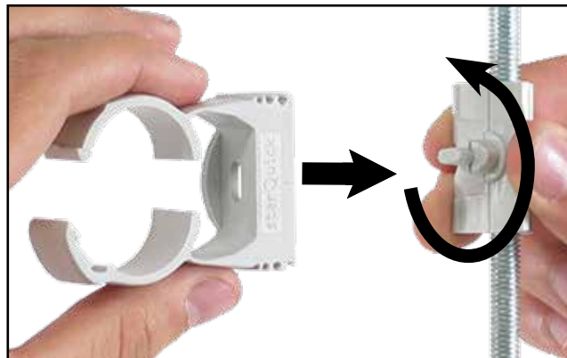
Close adapter and join clamp
