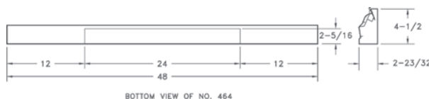
BOTTOM VIEW OF NO. 464
