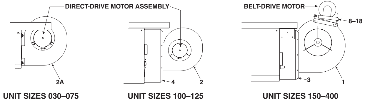
Figure 5. Blower Backs and Blowers (Refer to Table 13 and Table 14 )
