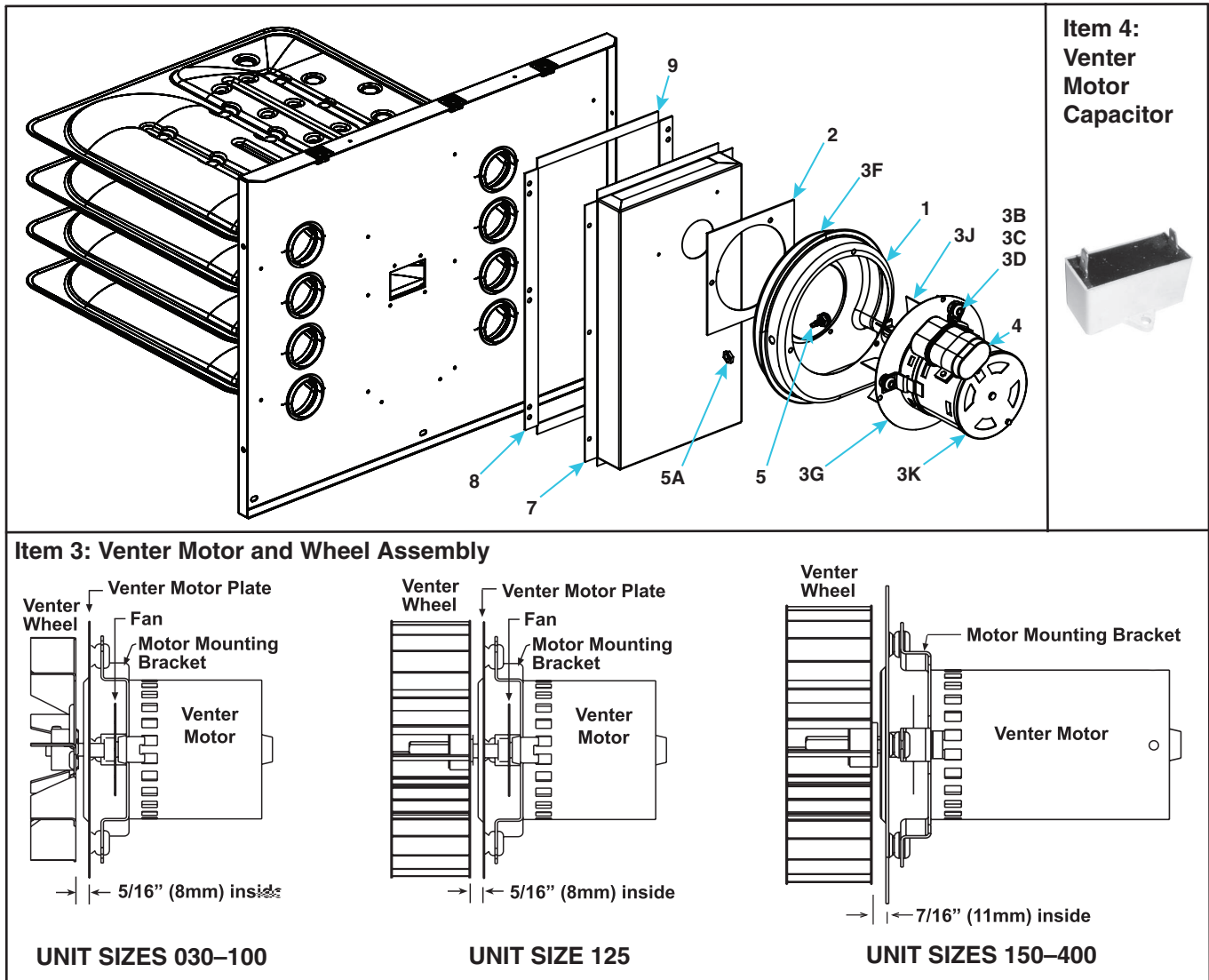
Figure 7. Venter and Flue Wrapper Components (Refer to Table 17 and Table 18 )
