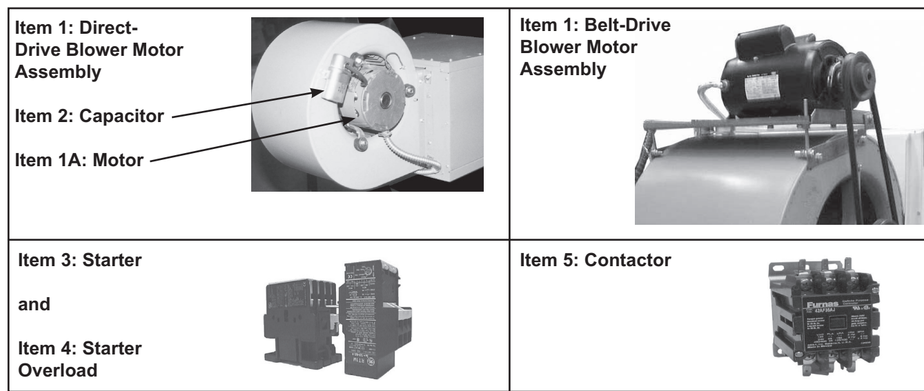
Figure 4. Individual Blower Components (Refer to Table 8 , Table 9 , and Table 10 )
