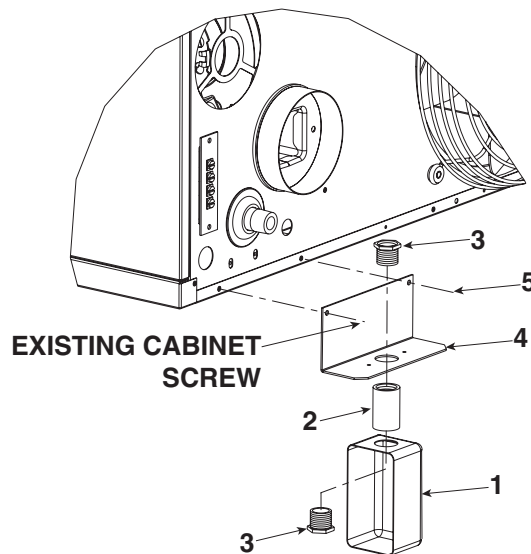
Figure 18. Thermostat Bracket Kit (Refer to Table 35)
