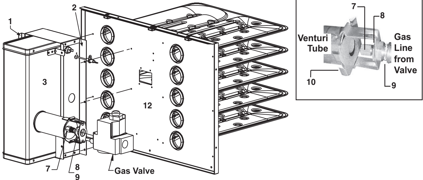
Figure 8. Replacement Heat Exchanger and Burner Assembly Components—Unit Sizes 030–125 (Refer to Table 19 and Table 20 )
