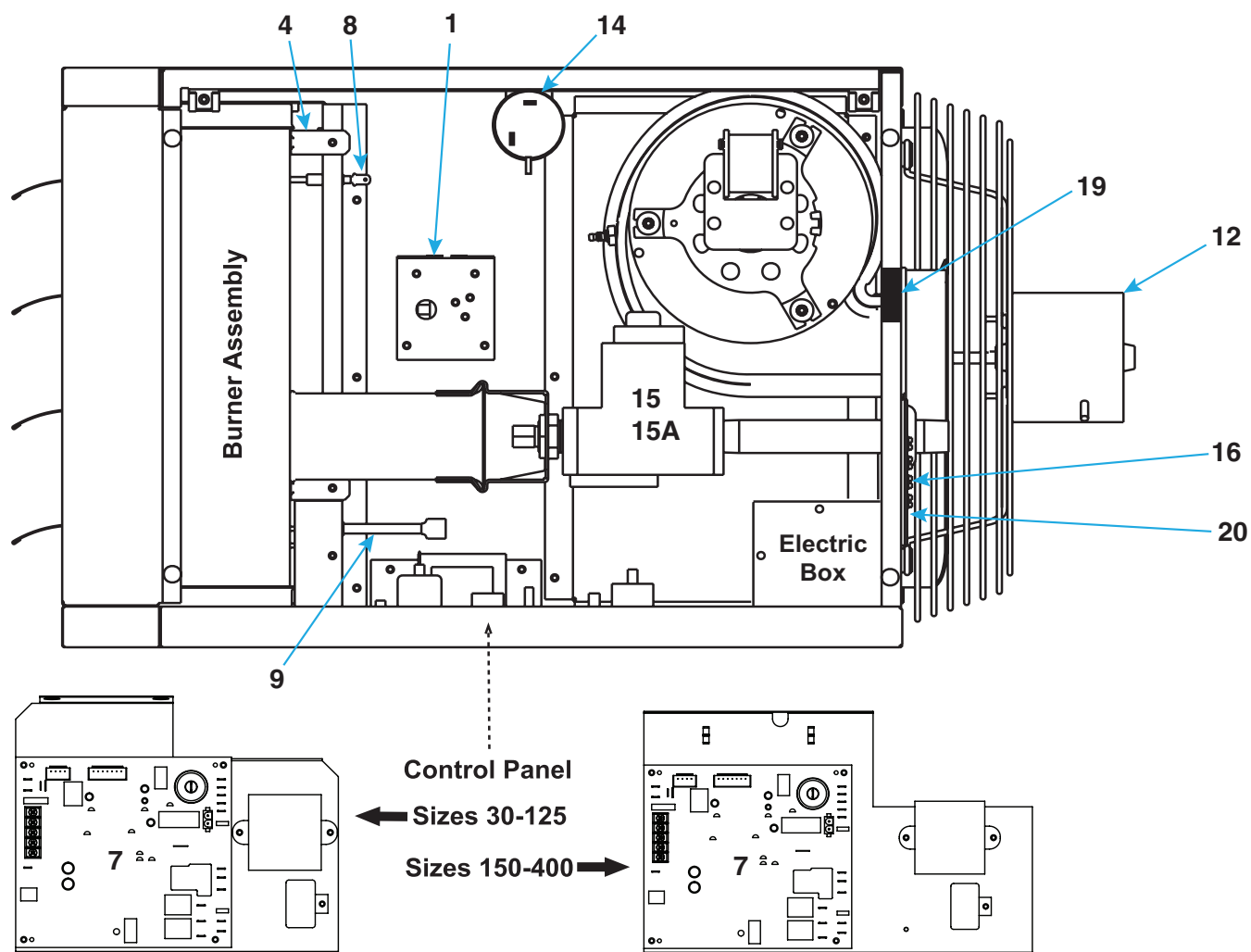
Figure 1. Typical Control Compartment (Refer to Table 4 and Table 5)
