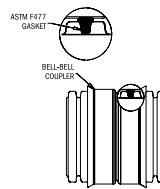
MEGA GREEN WT BELL-AND-SPIGOT
