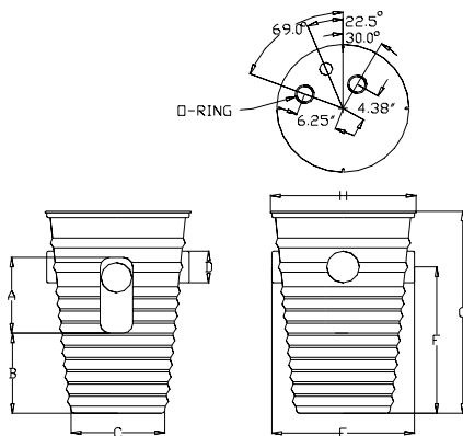
SEWAGE EJECTOR SUMP AND LID
