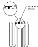
4"-10" (100-250mm) N-12 WT BELL-AND-SPIGOT
