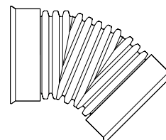
45° MITERED BEND N-12 ST AND N-12 WT
