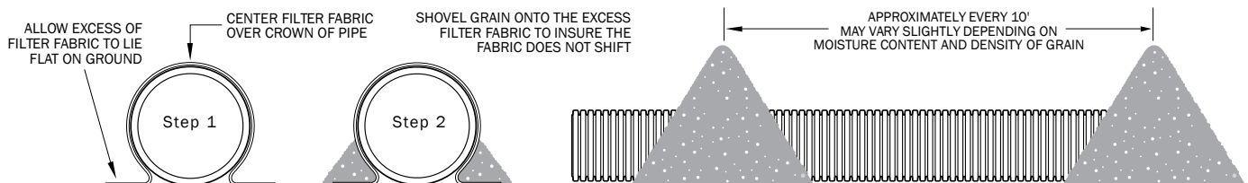
GRAIN-AIRE PIPE
