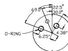
NON-LOCKING LID KIT FOR SEWAGE EJECTOR & RADON SUMP
