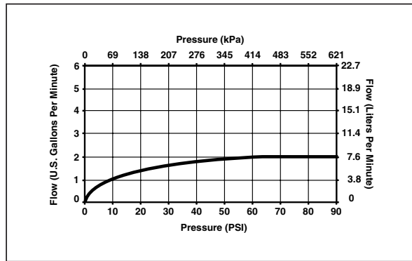
84001 Body Jet and 84110 Body Spray Flow Rate
